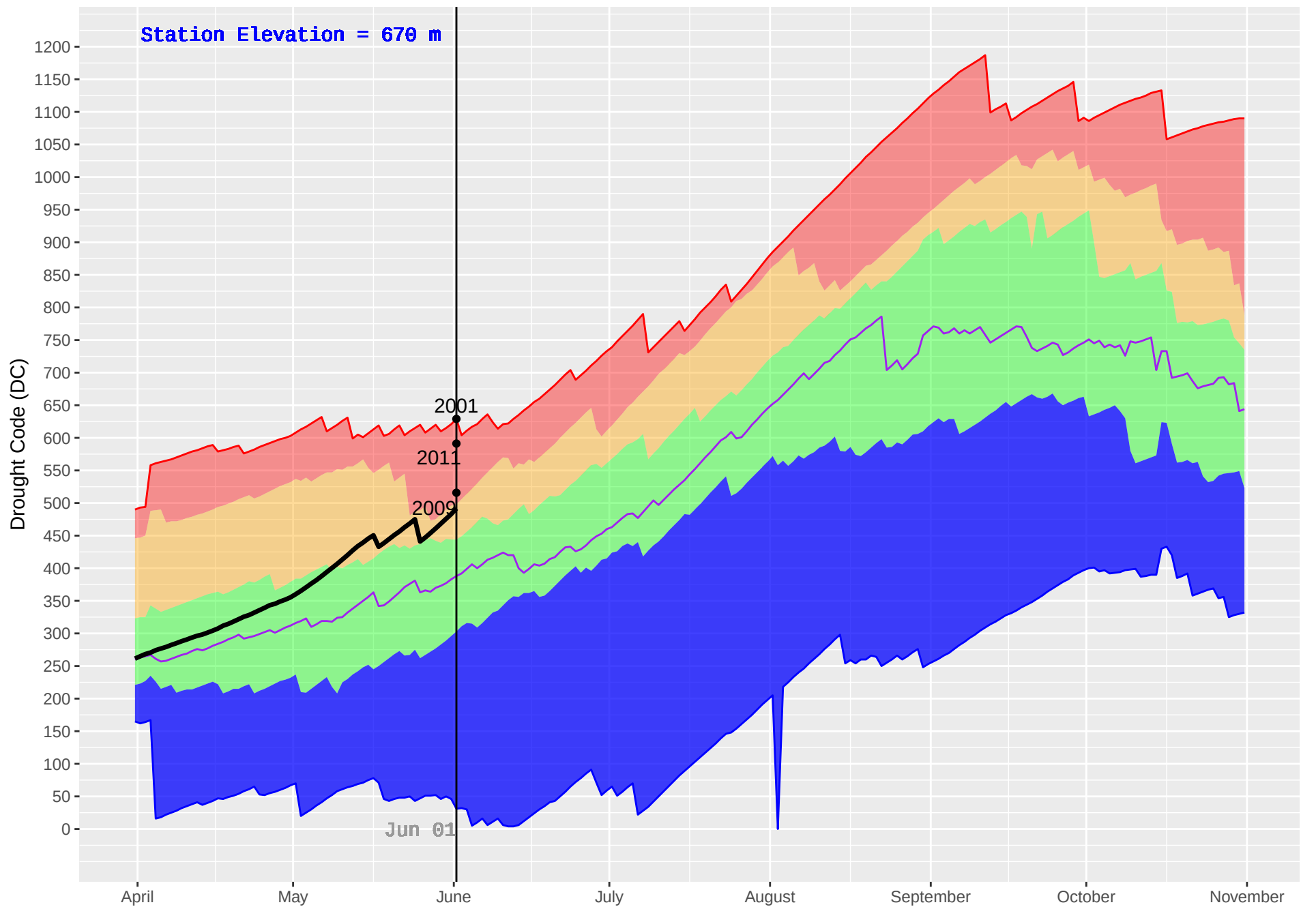
FINTRY (298) : Historical (1989–2018) and Current (2019) Daily Drought Code (DC)
