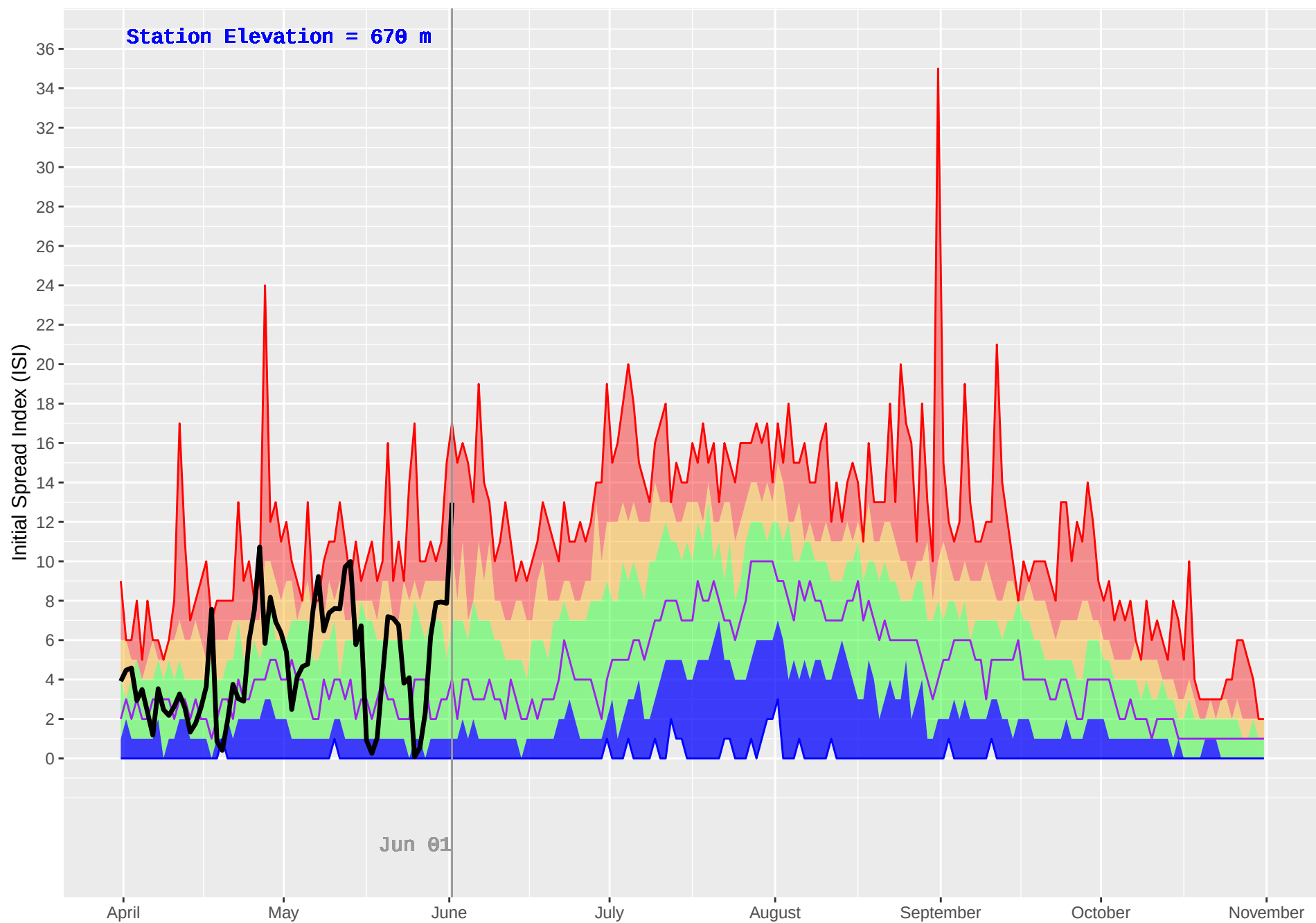
FINTRY (298) : Historical (1989–2018) and Current (2019) Daily Initial Spread Index (ISI)
