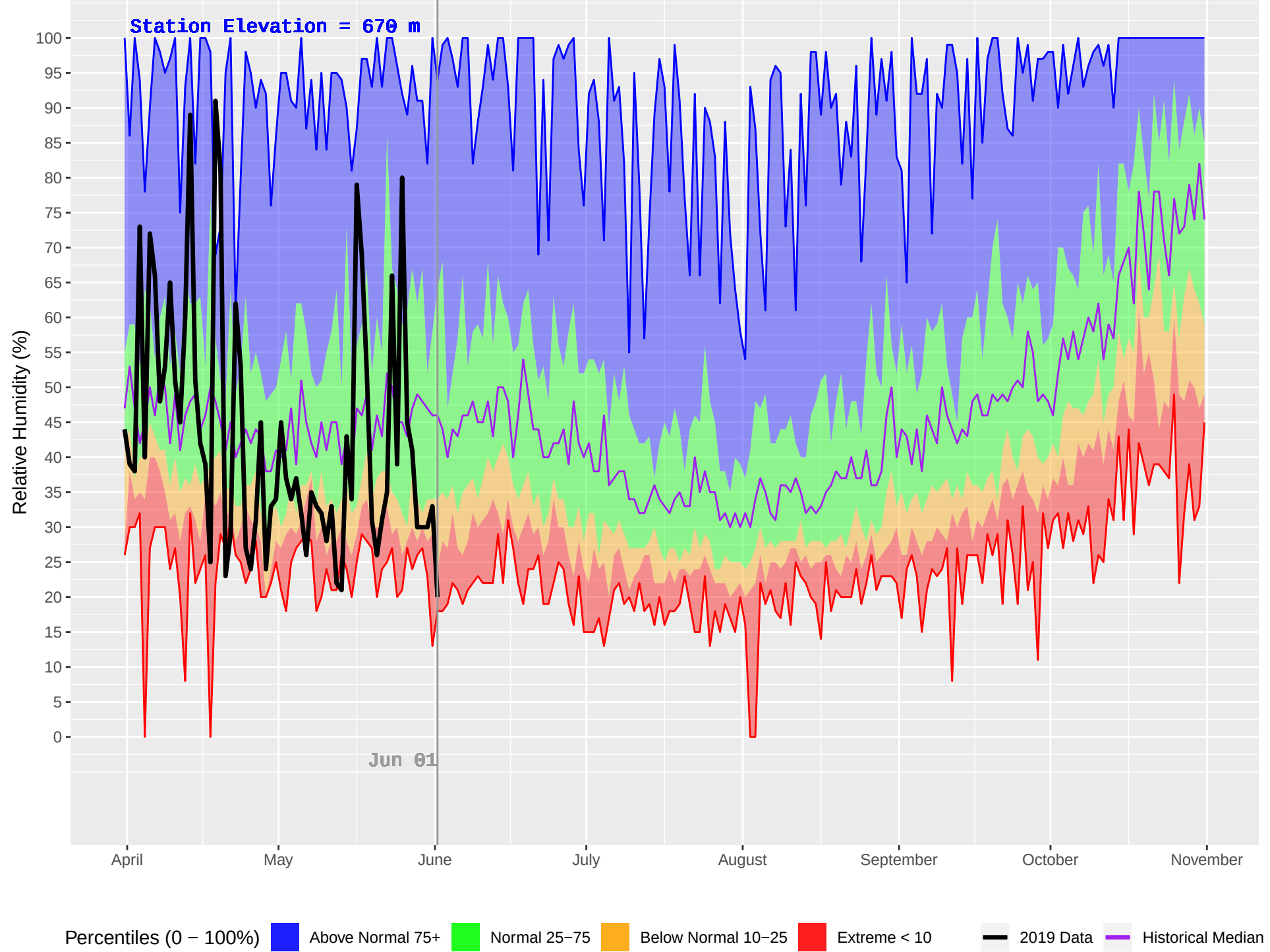
FINTRY (298) : Historical (1989–2018) and Current (2019) Daily Relative Humidity
