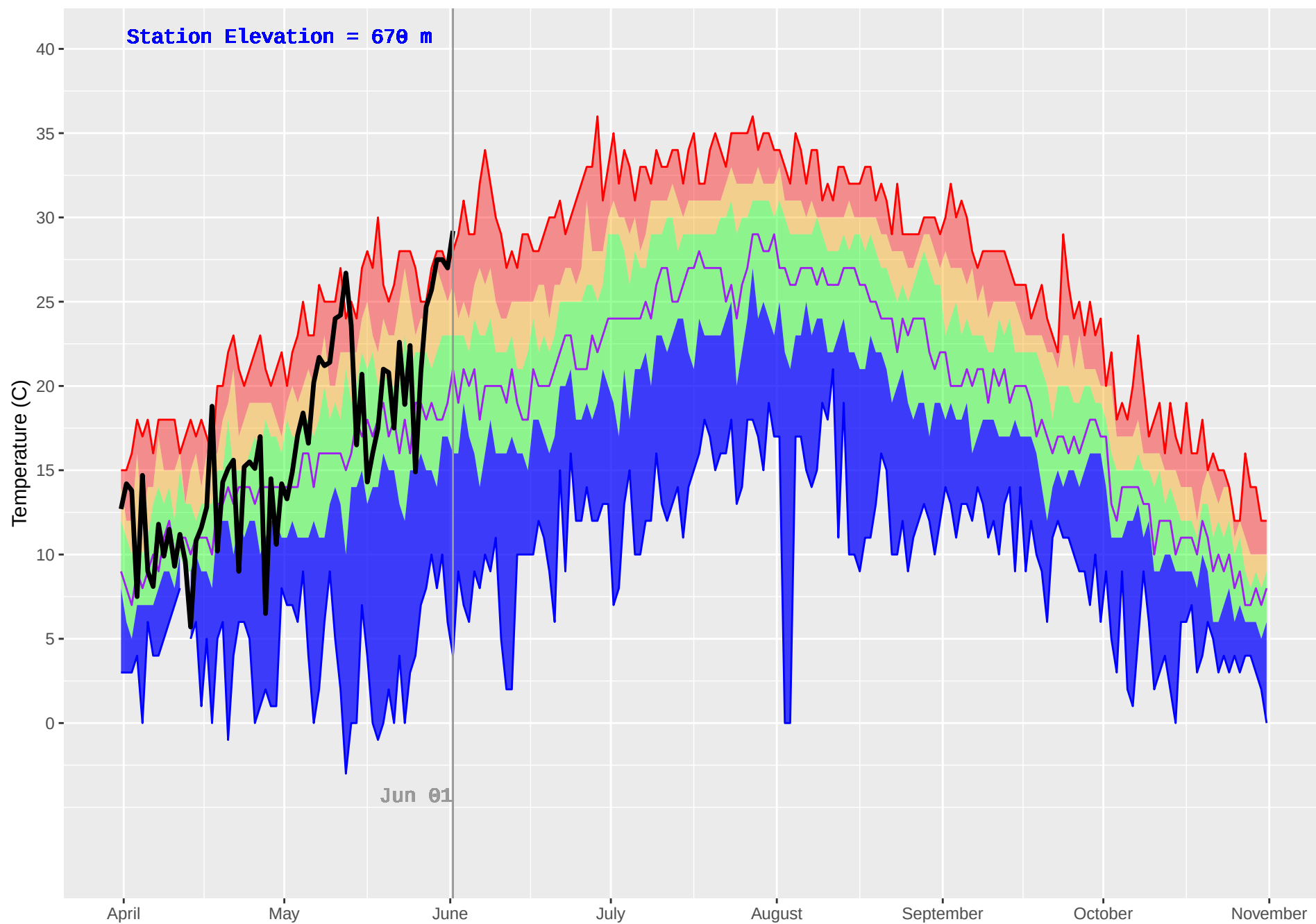
FINTRY (298) : Historical (1989–2018) and Current (2019) Daily Temperature
