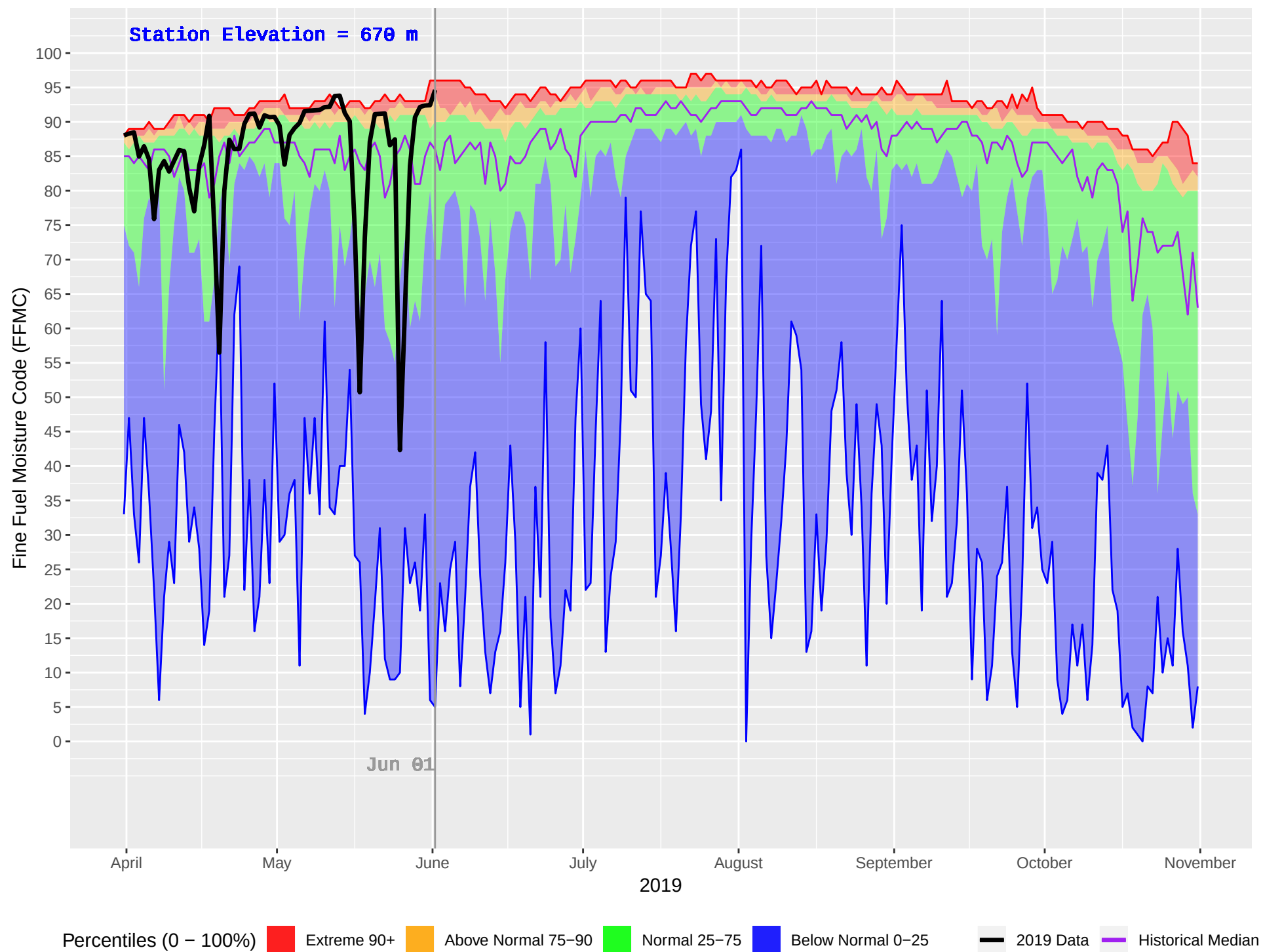
FINTRY (298) : Historical (1989–2018) and Current (2019) Daily Fine Fuel Moisture Code (FFMC)
