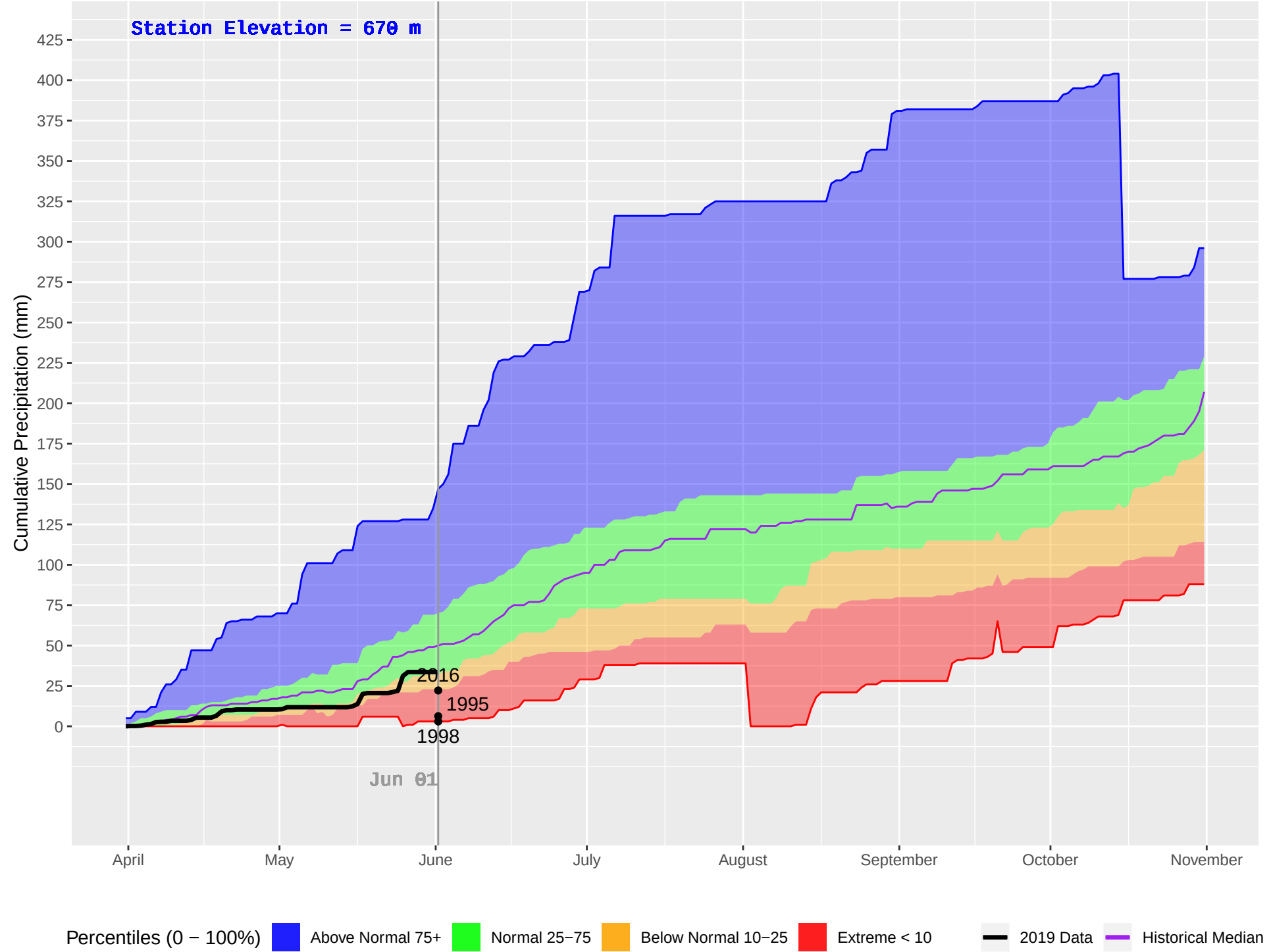
FINTRY (298) : Historical (1989–2018), Current (2019) Daily Cumulative Precipitation
