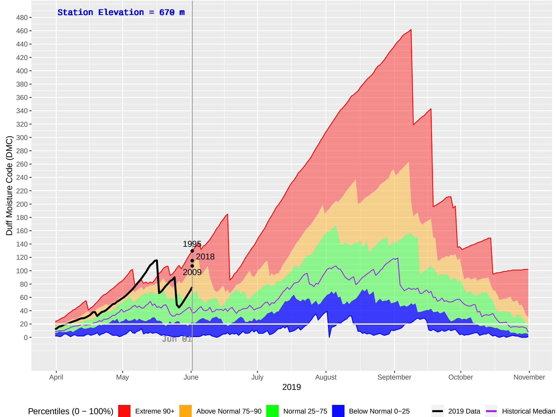
FINTRY (298) : Historical (1989–2018), Current (2019) Daily Duff Moisture Code (DMC)
