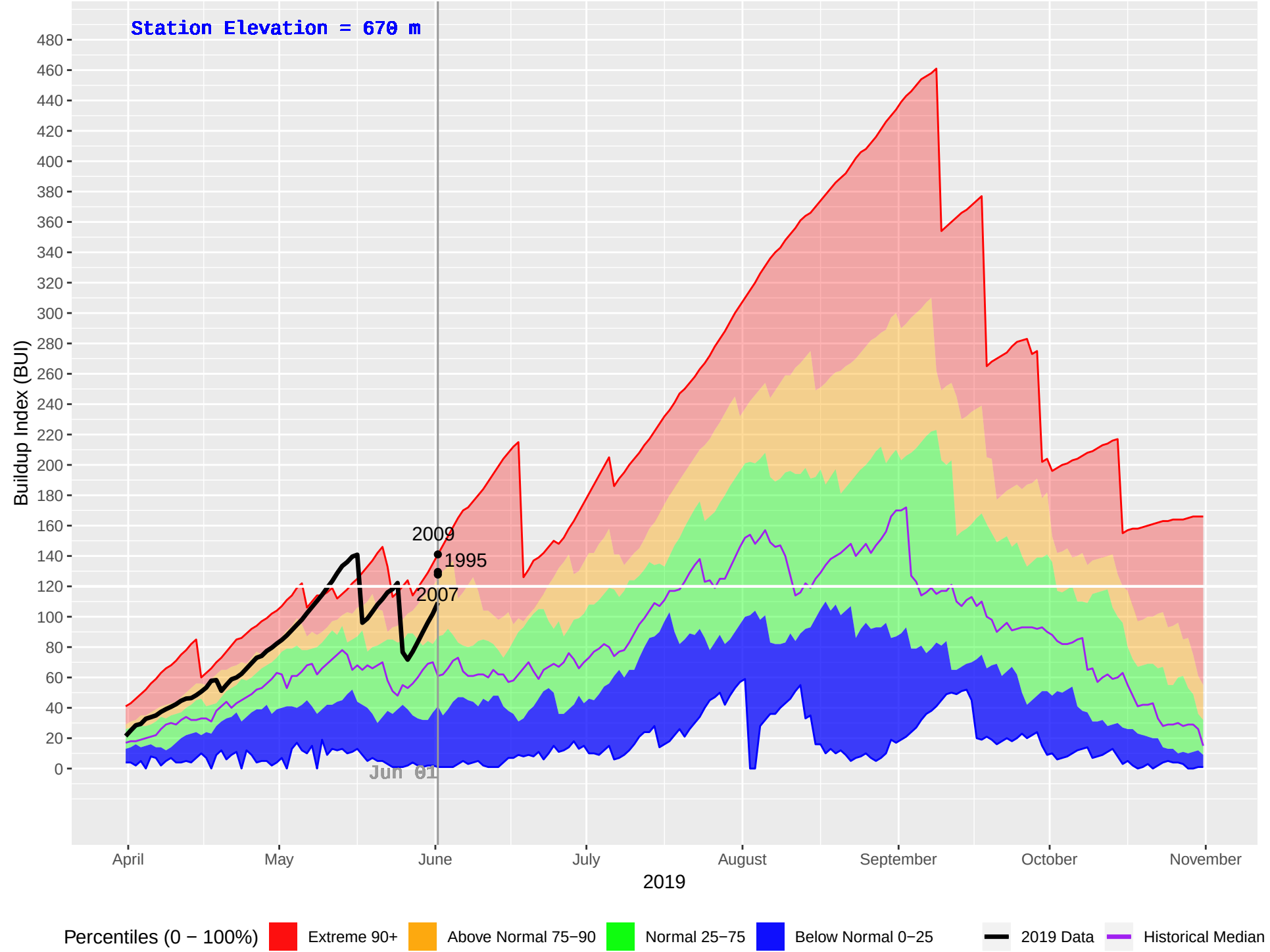
FINTRY (298) : Historical (1989–2018), Current (2019) Daily Buildup Index (BUI)
